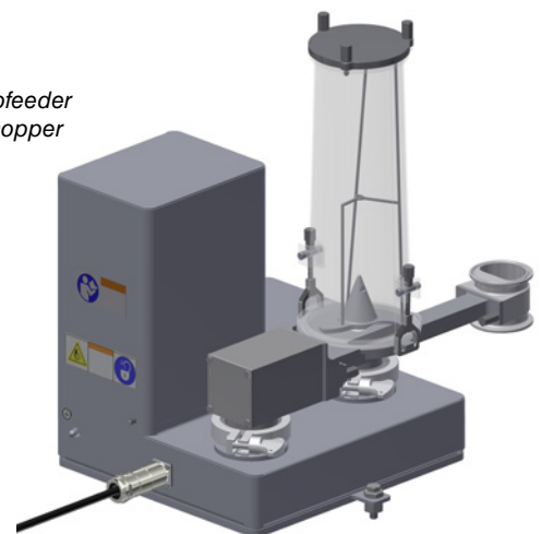
above: 12mm Microfeeder with 2 liter hopper and optional impactor
